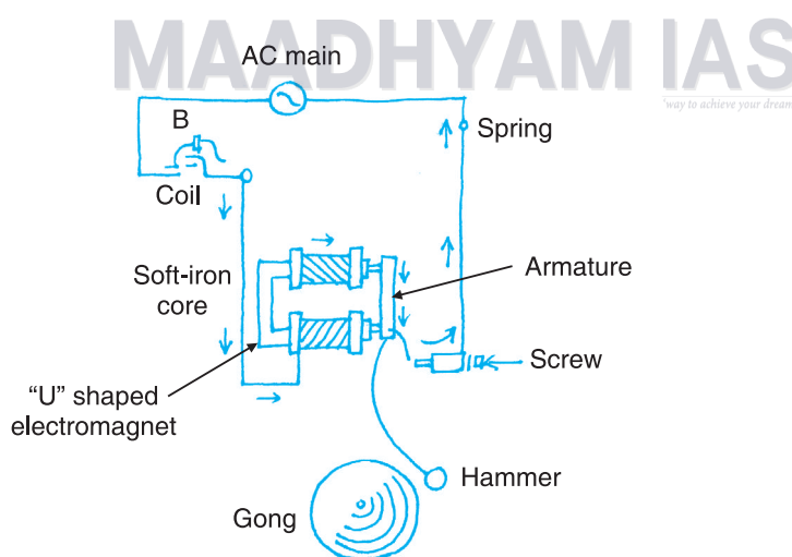
Fig. 17.9 Electric bell
