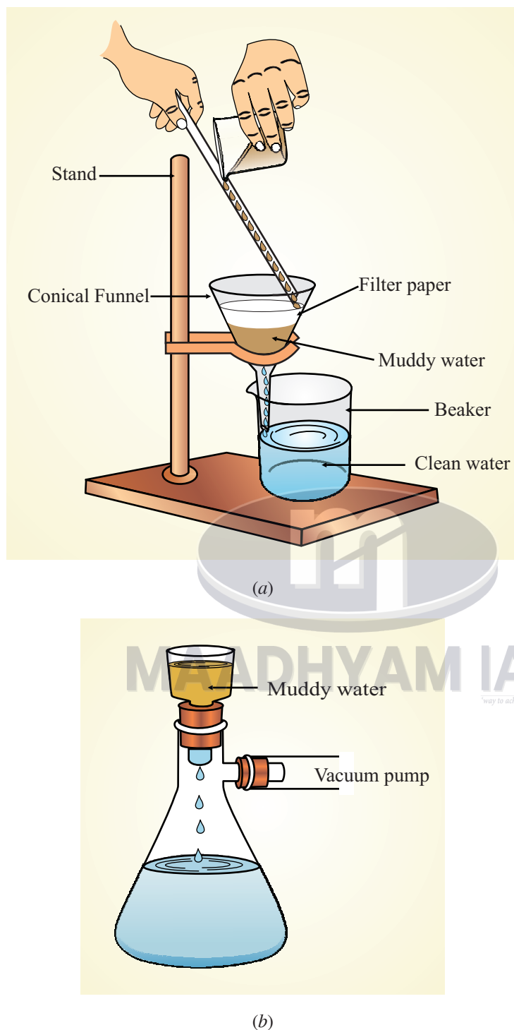
Fig. 2.13: Filtration (a) simple filtration (b) vacuum filtration
