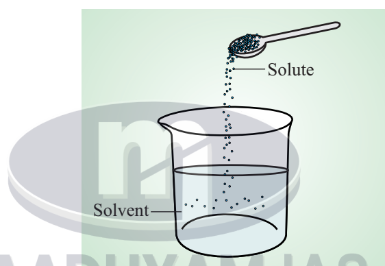
Fig. 2.10 Mixing of NaCl into water
