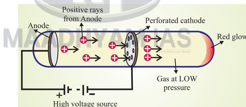
Fig. 5.3 Goldstein's cathode ray tube with perforated cathode
