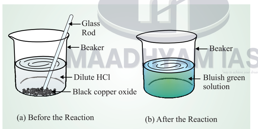
Fig. 8.3 Reaction between dilute hydrochloric acid and copper oxide (a) before reaction black particles of copper oxide in transparent dilute hydrochloric acid and (b) after reaction bluish green solution.
